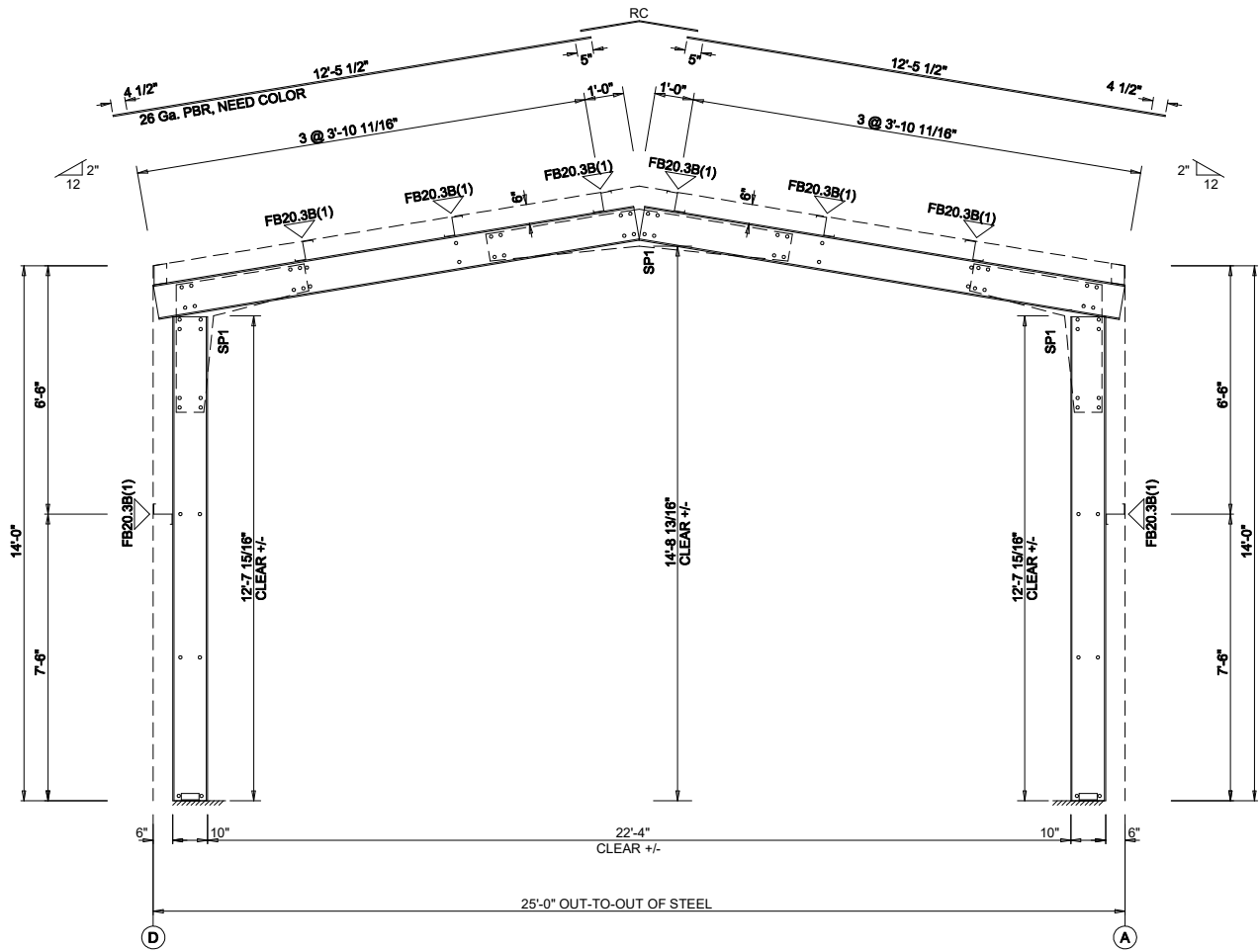
RIGID FRAME ELEVATION: FRAME LINE 2 3
