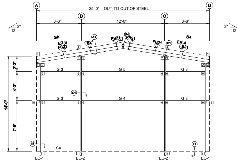
ENDWALL FRAMING: FRAME LINE 4
