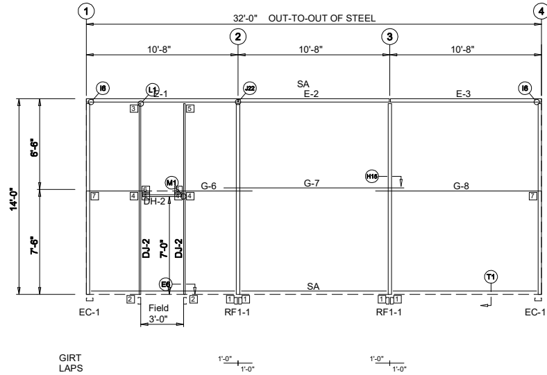
SIDEWALL FRAMING: FRAME LINE A
