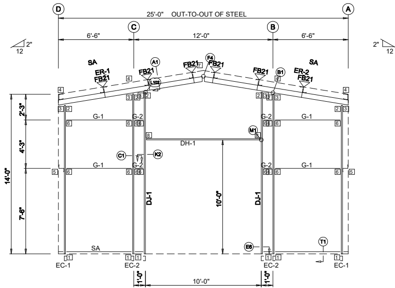
ENDWALL FRAMING: FRAME LINE 1
