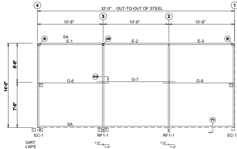
SIDEWALL FRAMING: FRAME LINE D
